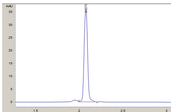
Figure 3. A representative chromatogram for the quantification of the vancomycin concentration in a dialysate.
